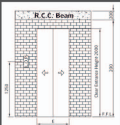
Center Opening Auto Door
