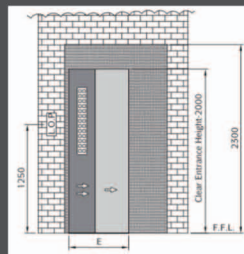
Telescopic Door (two fold)
